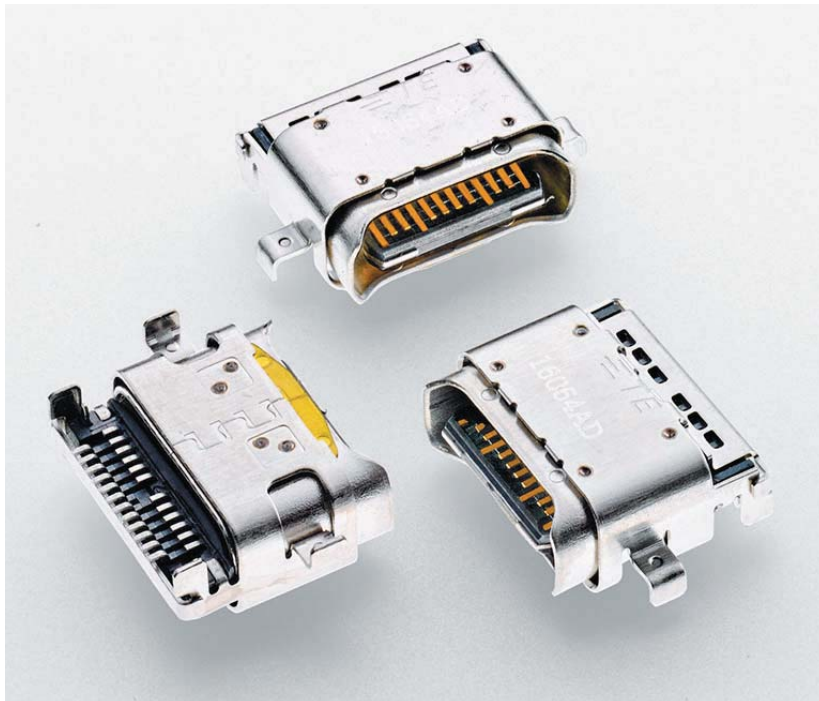
Rugged USB Type-C connectors with IPX8 waterproof ratings are a useful choice for outdoor surveillance devices.
